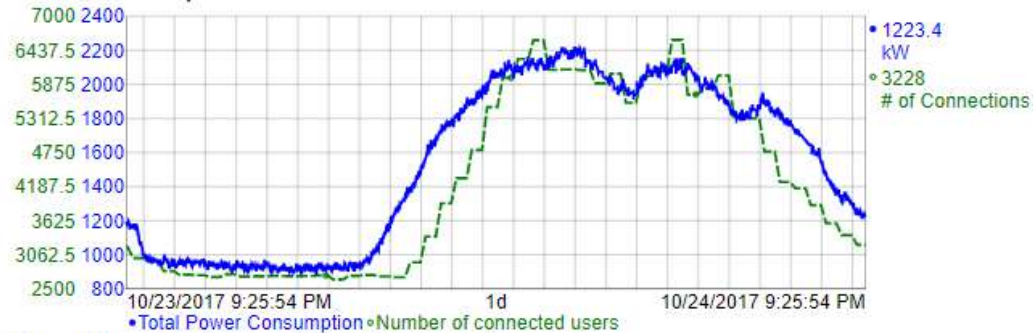
Power Consumption vs Users Connected.
